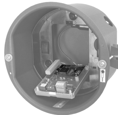
TXB-V TRANSLATOR BOARD (SHOWN INSTALLED WITH SPECTRA BACK BOX)
