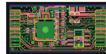
HDMI PCB
