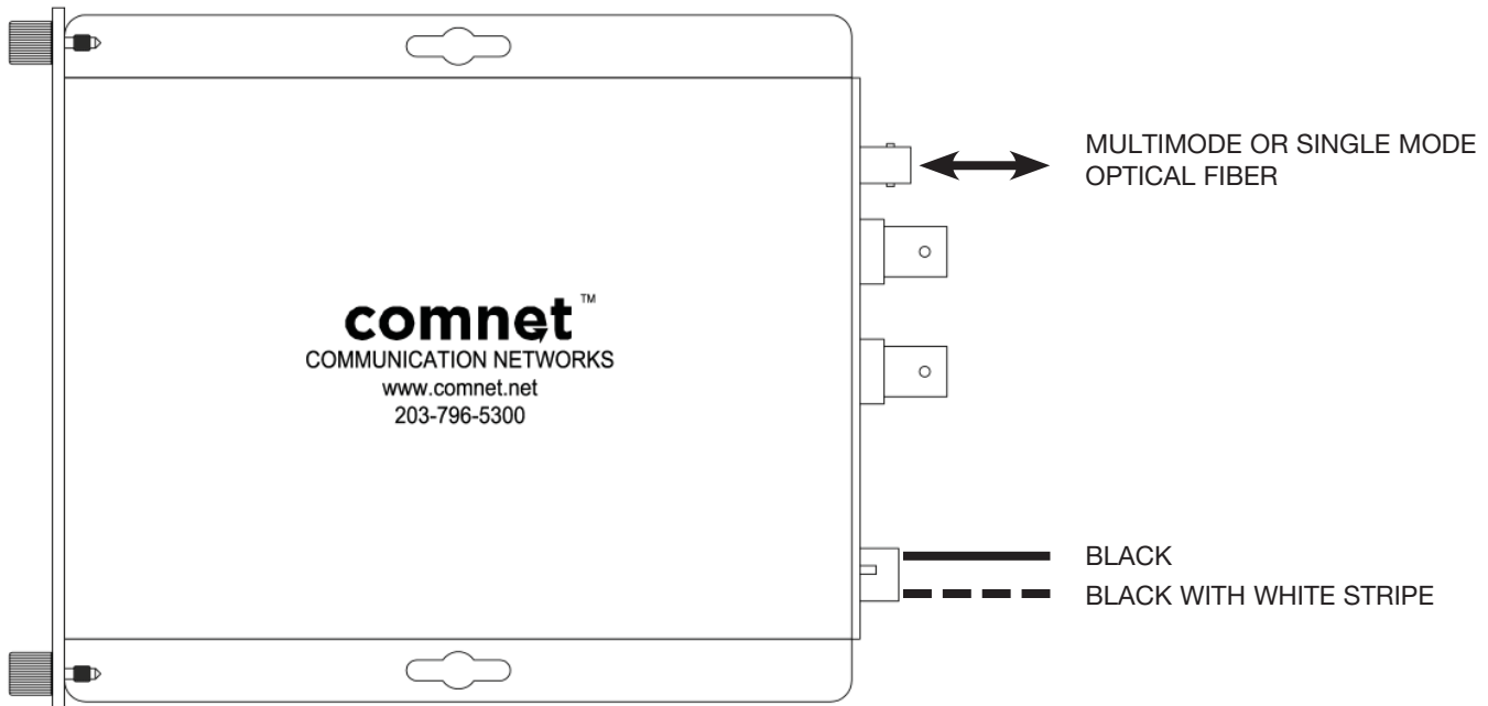
FIGURE 1 – FVTR TRANSCEIVER
