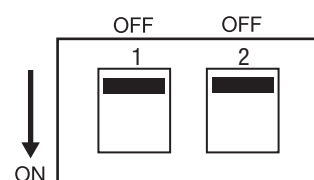
4) RS-485, 4-WIRE DATA
