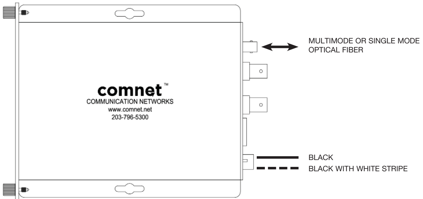
FIGURE 1 – FVTRD TRANSCEIVER
