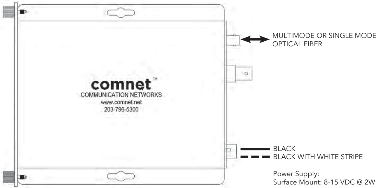
FIGURE 1 - FVT/FVR1001
