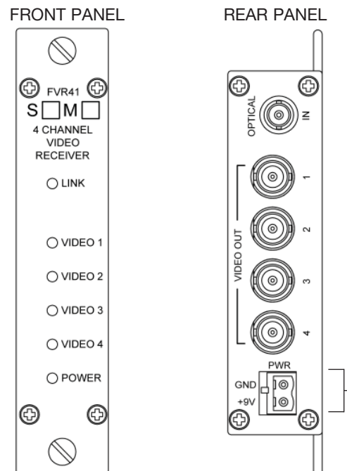
FIGURE 3 – FVR41 RECEIVER
