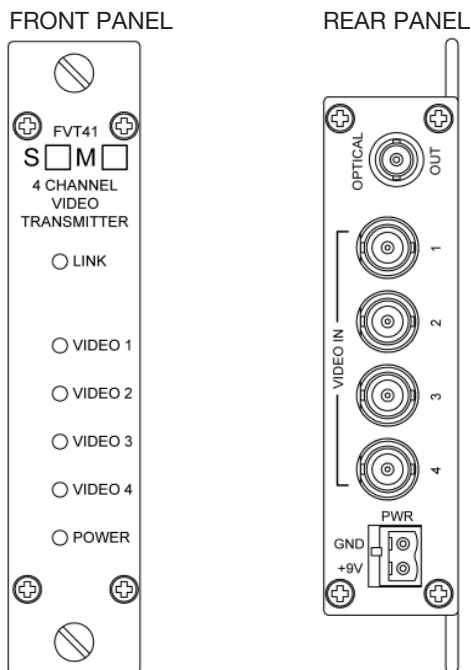
FIGURE 2 – FVT41 TRANSMITTER
