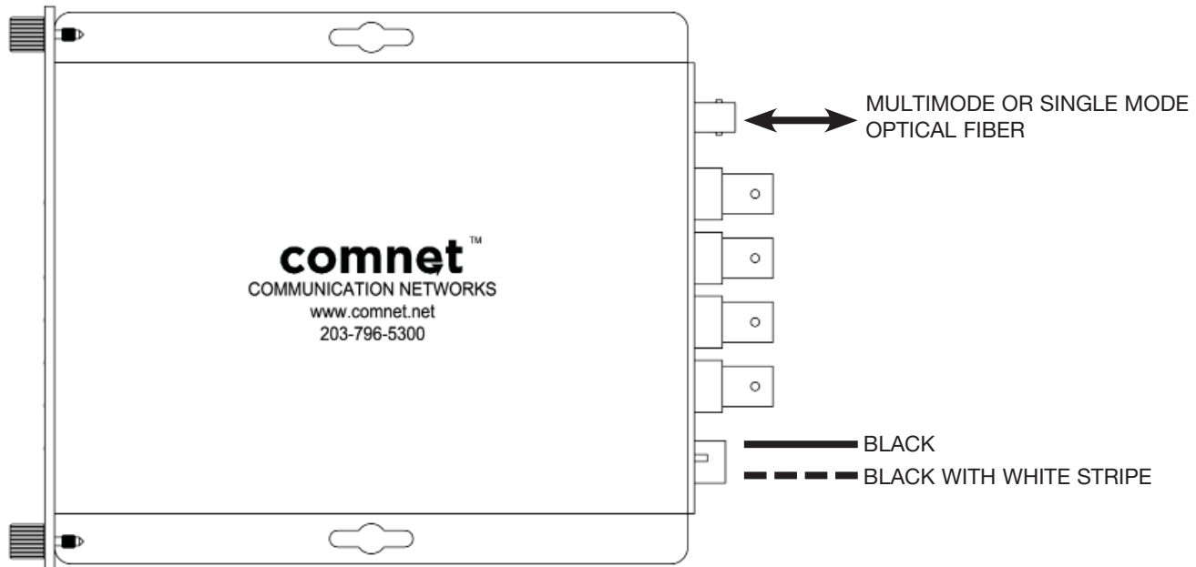
FIGURE 1 – FVT/FVR41 TRANSMITTER AND RECEIVER
