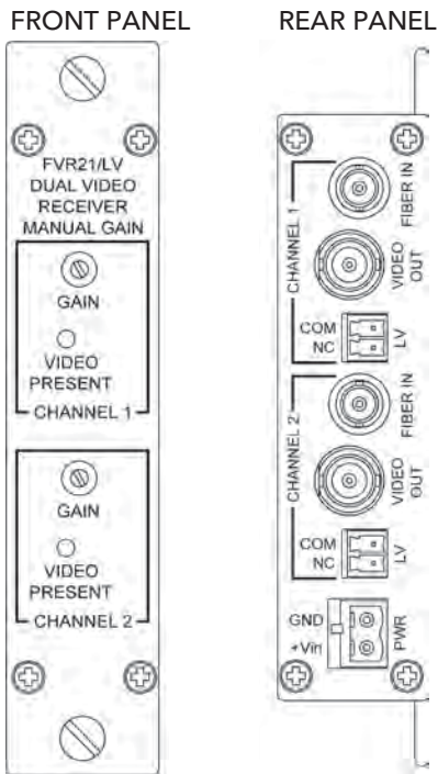
FIGURE 2 - FVR21 RECEIVER
