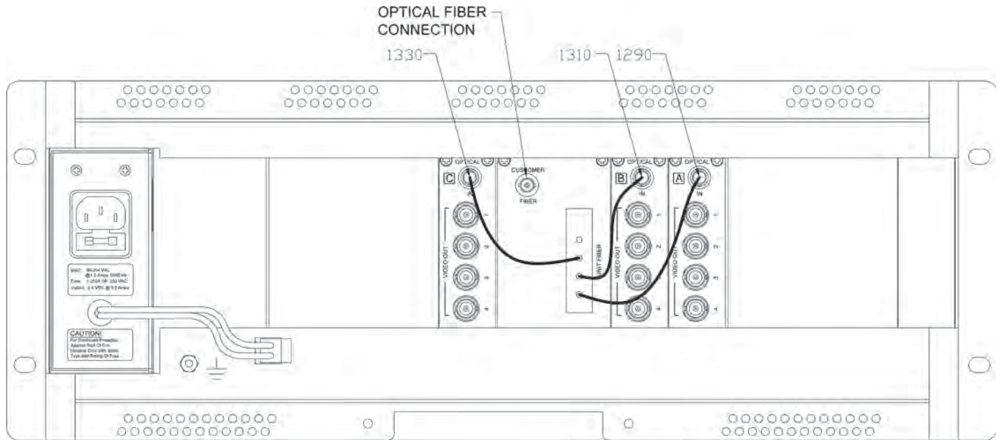
FIGURE 4 – FVR120M1 RECEIVER FRONT AND REAR
