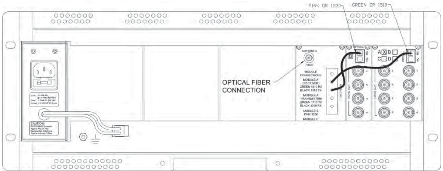
FIGURE 2 – FVR120S1 RECEIVER FRONT AND REAR
