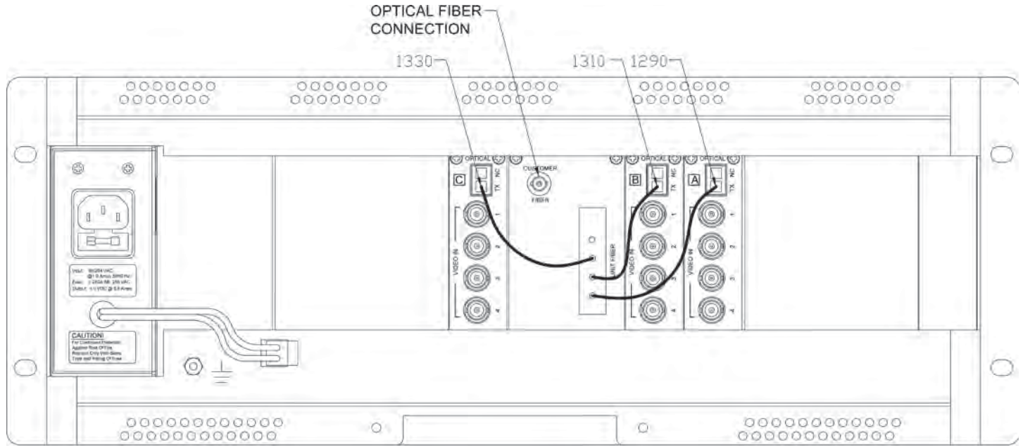
FIGURE 3 – FVT120M1 TRANSMITTER FRONT AND REAR
