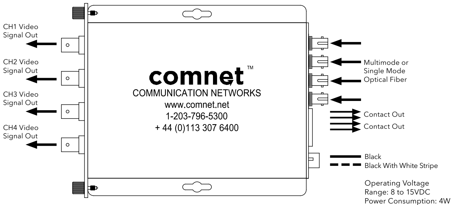
FIGURE 8 - FVR40C4 RECEIVER
