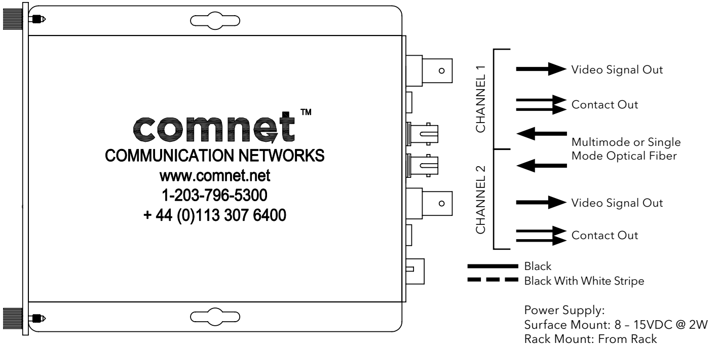
FIGURE 6 - FVR20C2 RECEIVER
