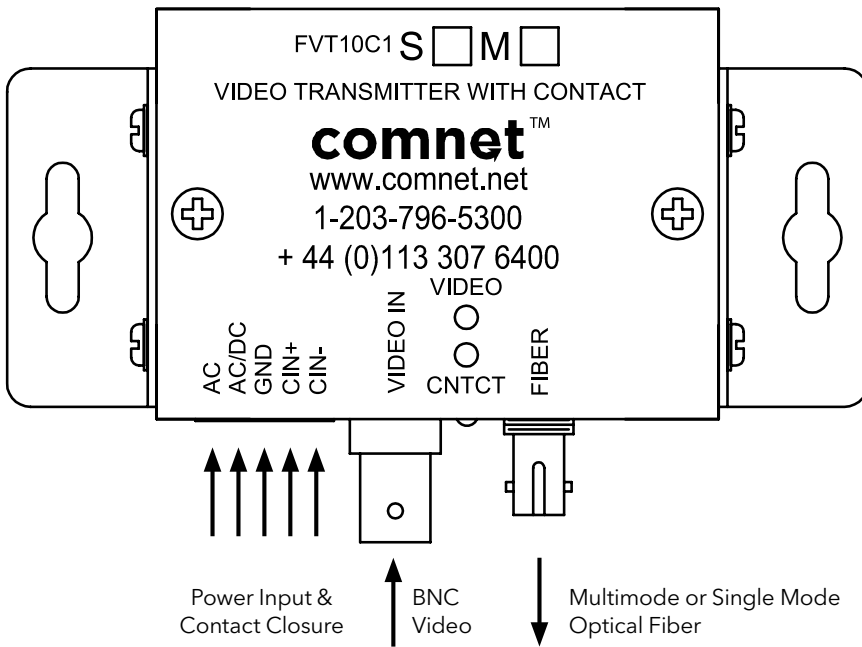
FIGURE 1 - FVT10C1/M TRANSMITTER
