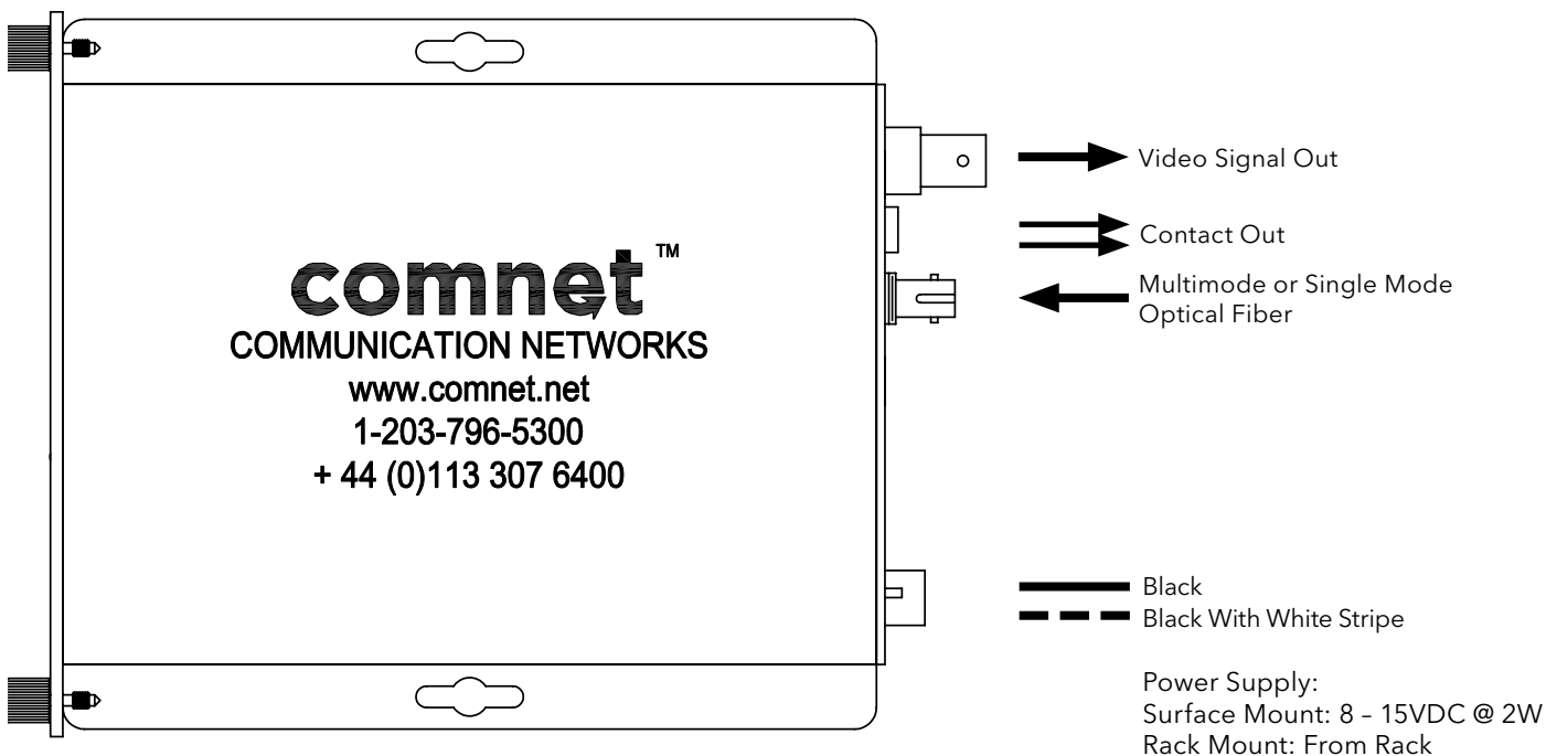
FIGURE 4 - FVR10C1 RECEIVER
