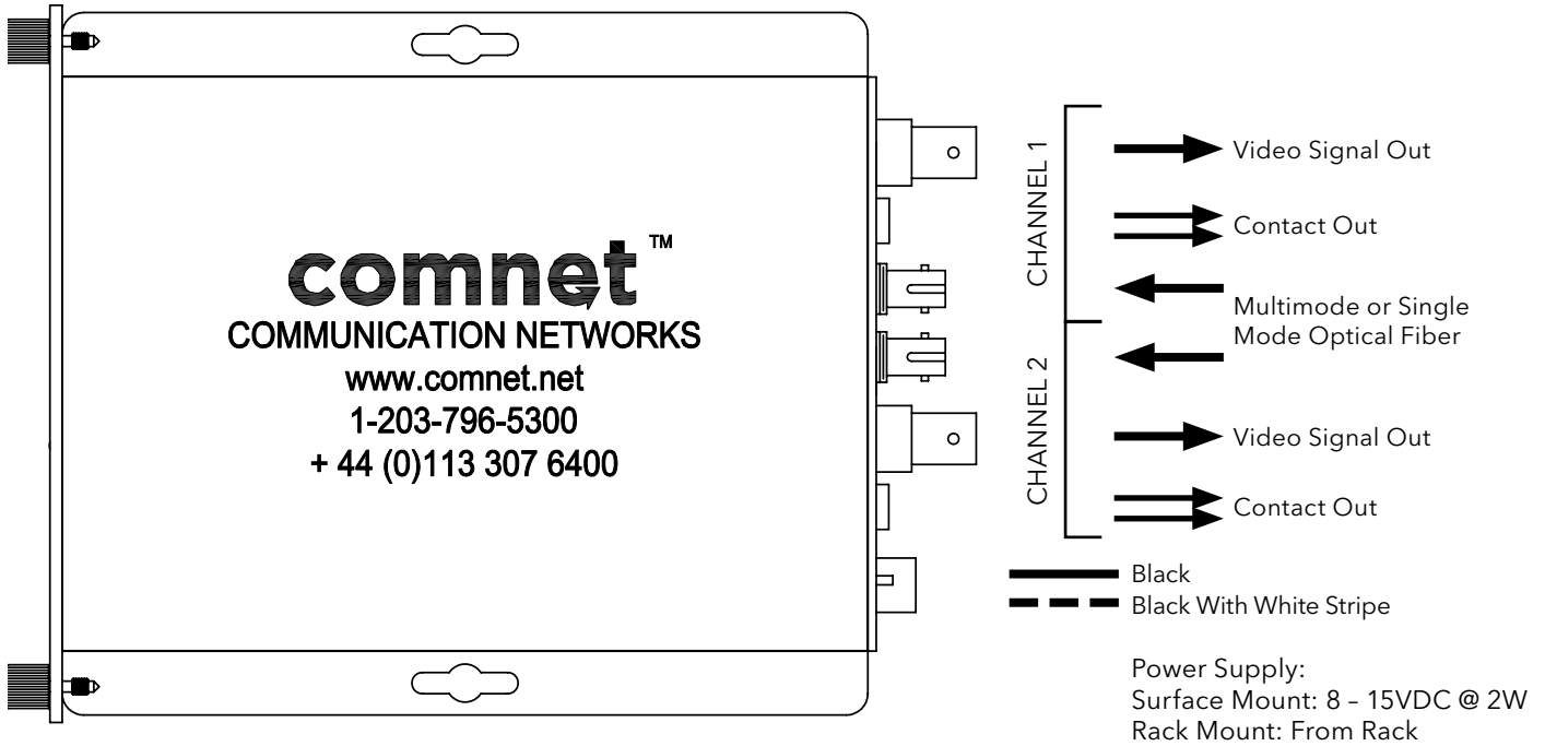
FIGURE 6 - FVR20C2 RECEIVER
