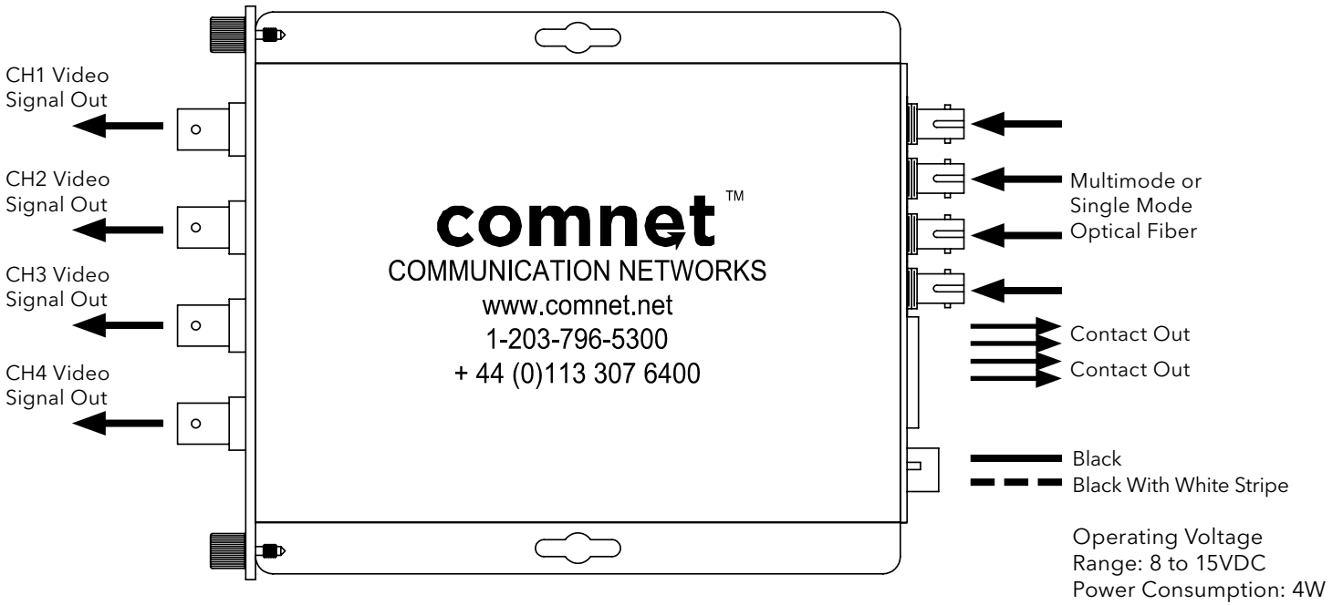
FIGURE 8 - FVR40C4 RECEIVER
