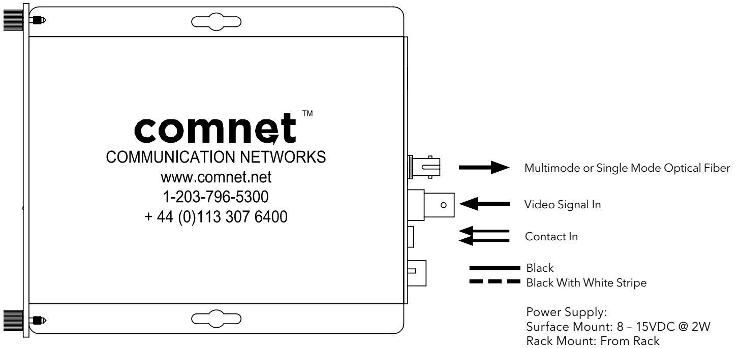
FIGURE 2 - FVT10C1 TRANSMITTER
