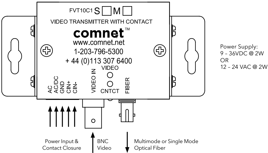
FIGURE 1 - FVT10C1/M TRANSMITTER
