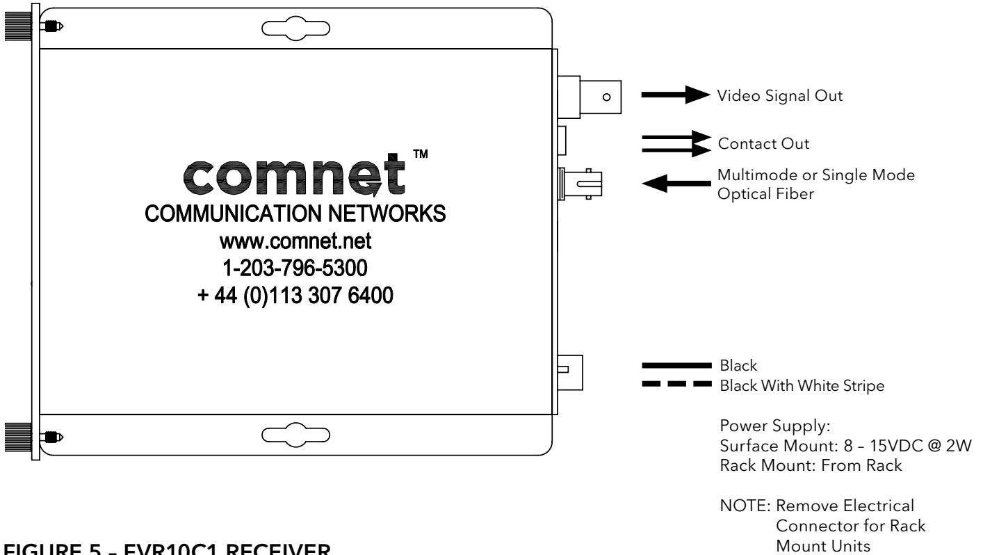
FIGURE 5 - FVR10C1 RECEIVER
