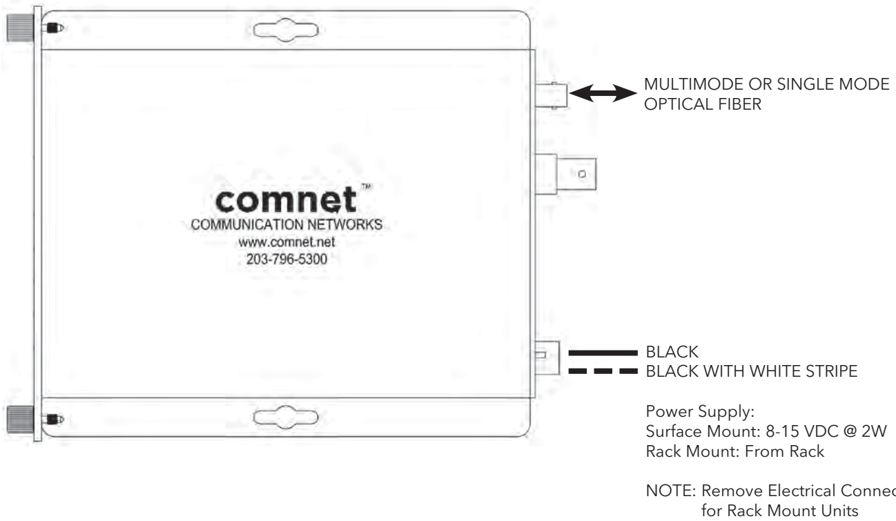
FIGURE 1 - FVT/FVR1001
