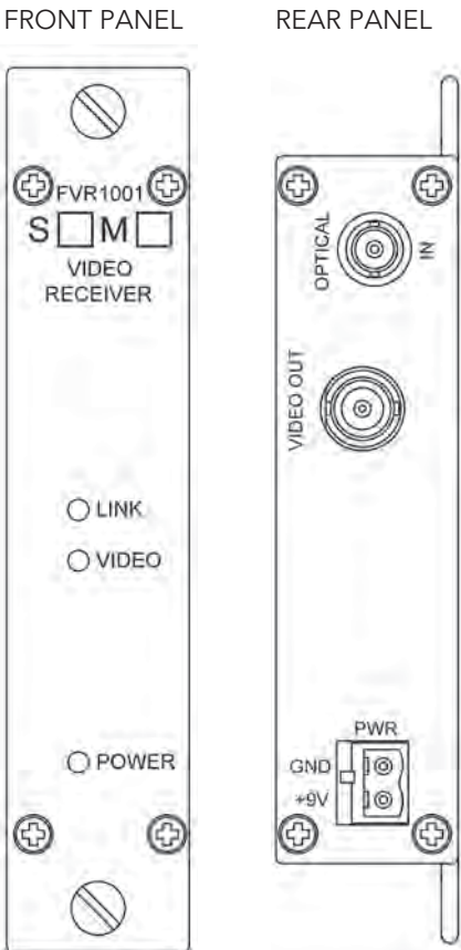
FIGURE 2 - FVR1001 RECEIVER
