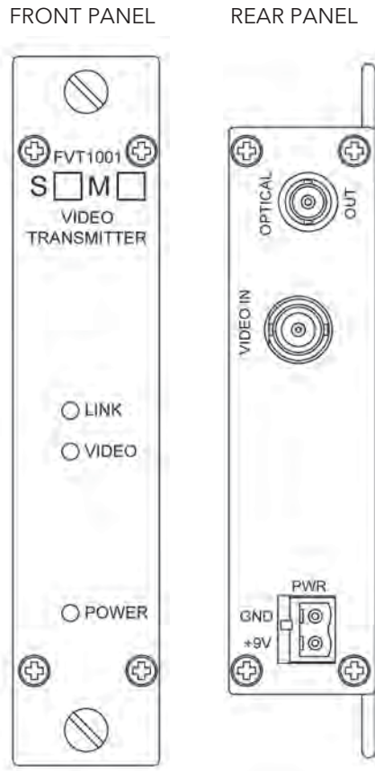
FIGURE 3 - FVT1001 TRANSMITTER
