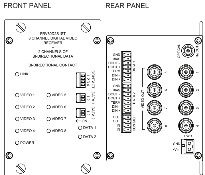
FIGURE 3 – RECEIVER
