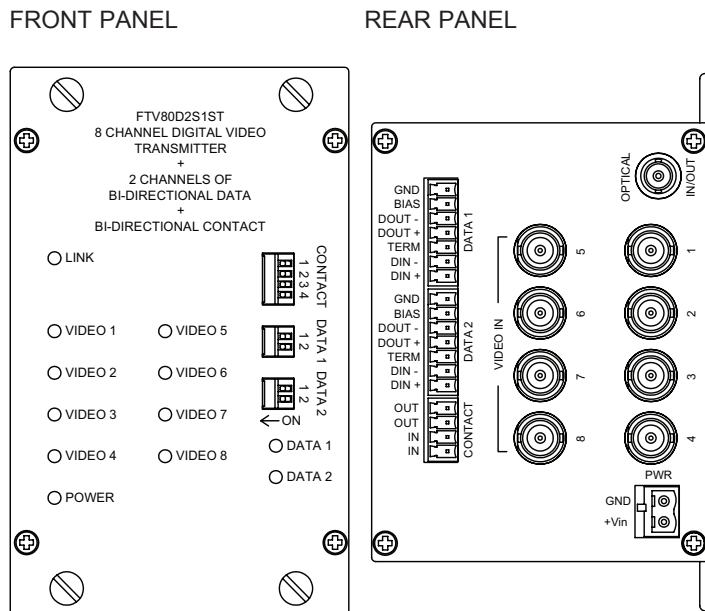
FIGURE 2 – TRANSMITTER
