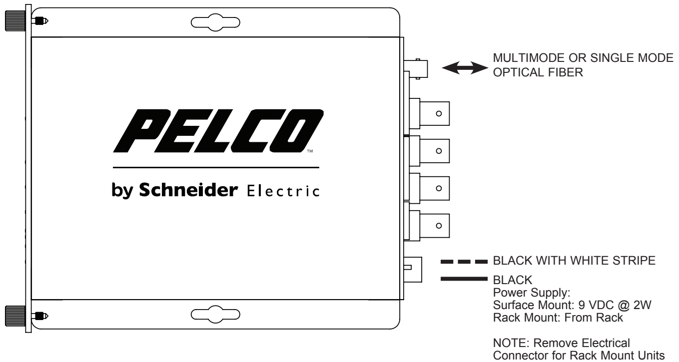
FIGURE 1 – FTV/FRV40D2(M,S)1(ST,FC) TRANSMITTER AND RECEIVER
