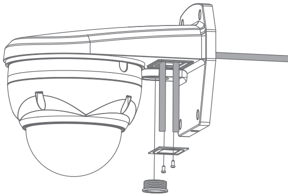
CABLE ASSEMBLY MODE
