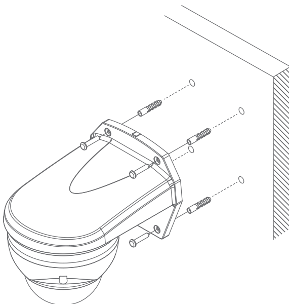
WALL MOUNT BRACKET ASSEMBLY MODE
