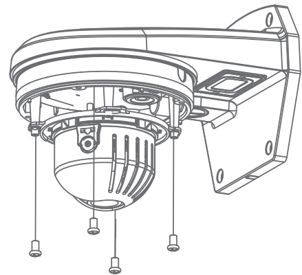
DOMES HOUSING ASSEMBLY MODE
