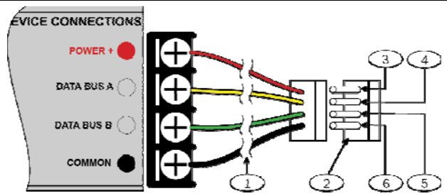
Figure 9: Bosch Control Panel to Keypad Flying Leads Wiring
