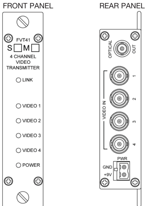
FIGURE 2 – FVT41 TRANSMITTER
