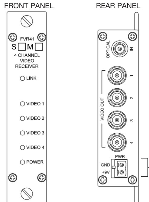
FIGURE 3 – FVR41 RECEIVER
