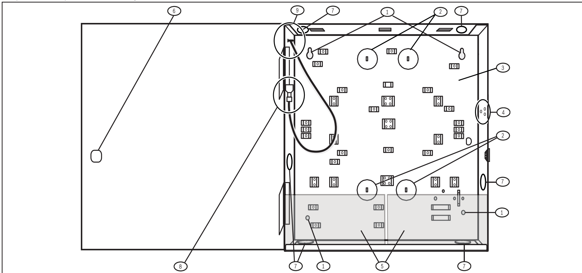
Figure 1.1: B10 Medium Control Panel Enclosure overview
