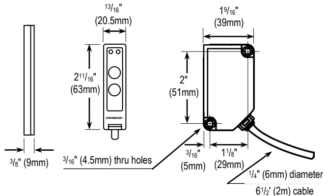
Transmitter/Receiver
