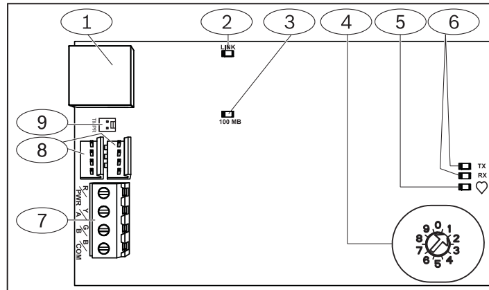
Figure 1.1: Board overview
