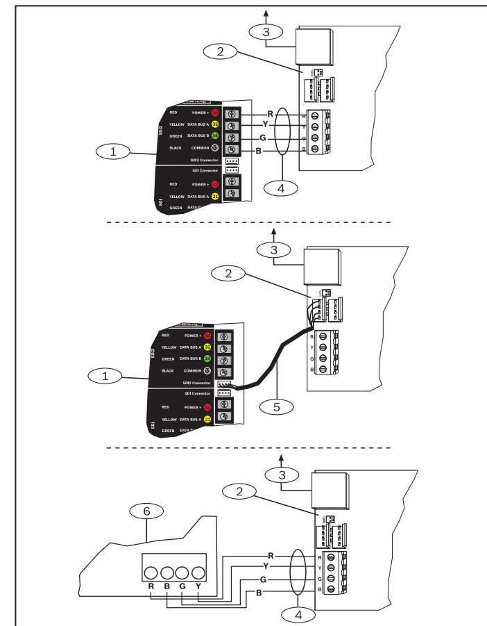
Figure 3.2: Wiring to the control panel (GV4 Series and FPD-7024 control panel shown)
