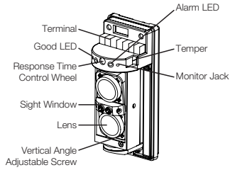
Receiver
