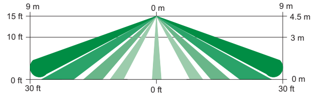
AR13-18 Side View 360° x 18 m (60 ft) diameter
