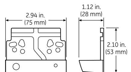
Sensor module with mounting bracket
